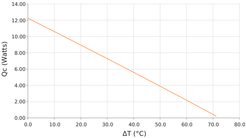
Heat Pumped at Cold Side (Qc) Thot = 35 °C | Ioperating = 2.6 Amps
