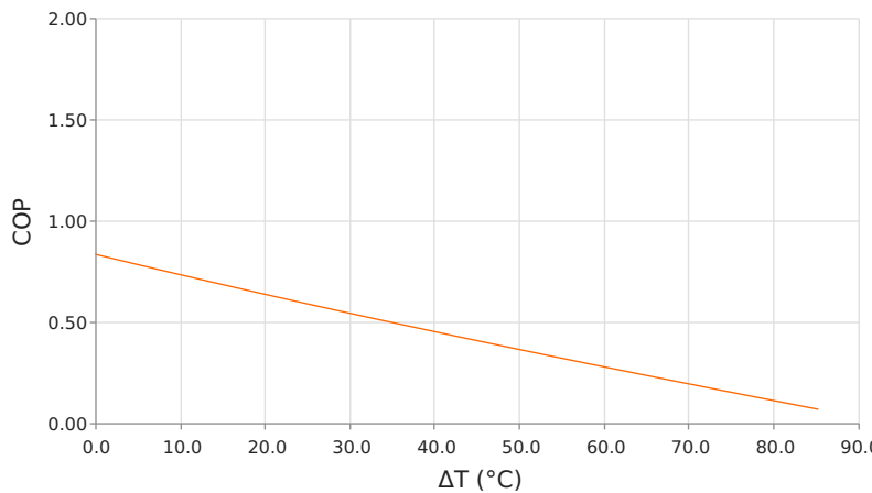
Coefficient of Performance (COP = Q_c/P_{in} ) T_{hot} = 85\text{ }^{\circ}\text{C} | operating = 2.9 Amps
