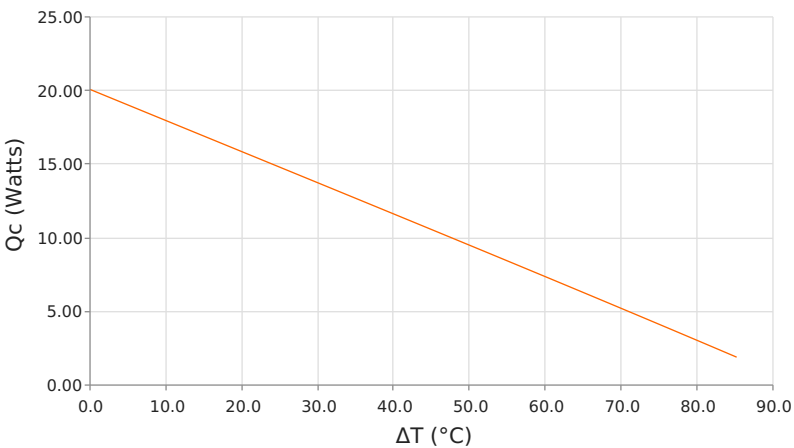
Heat Pumped at Cold Side ( Q_c ) T_{hot} = 85\text{ }^{\circ}\text{C} | operating = 2.9 Amps
