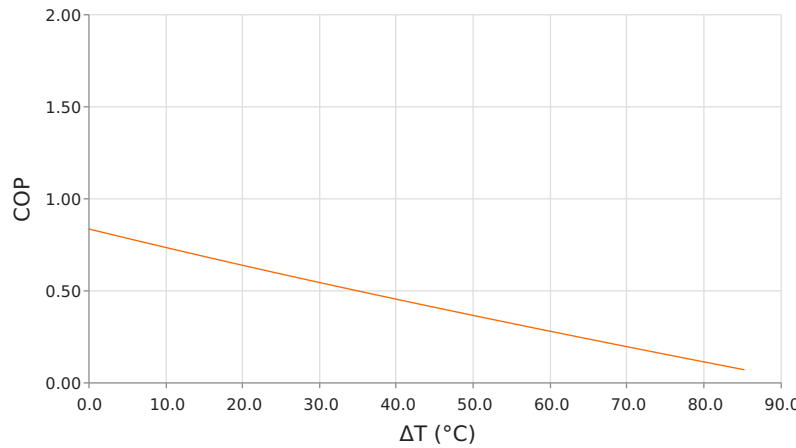
Coefficient of Performance (COP = Q_c/P_{in} ) T_{hot} = 85^\circ\text{C} | operating = 4.2 Amps
