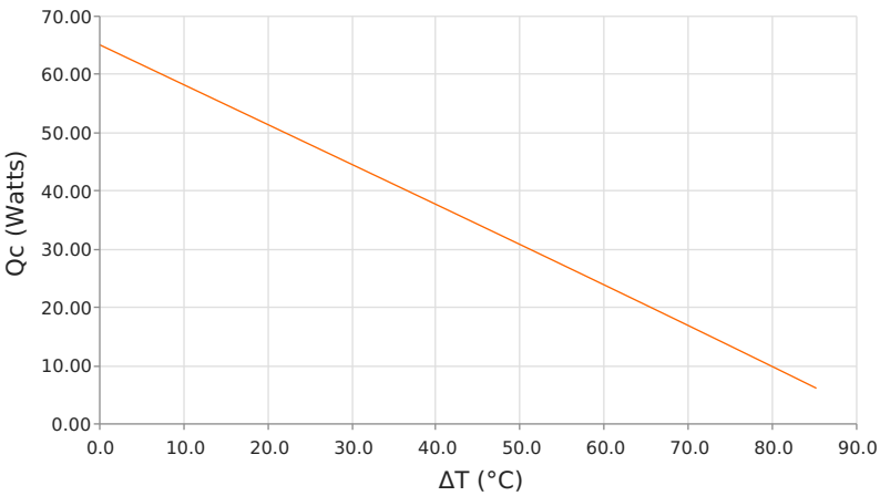
Heat Pumped at Cold Side ( Q_c ) T_{hot} = 85^\circ\text{C} | operating = 4.2 Amps
