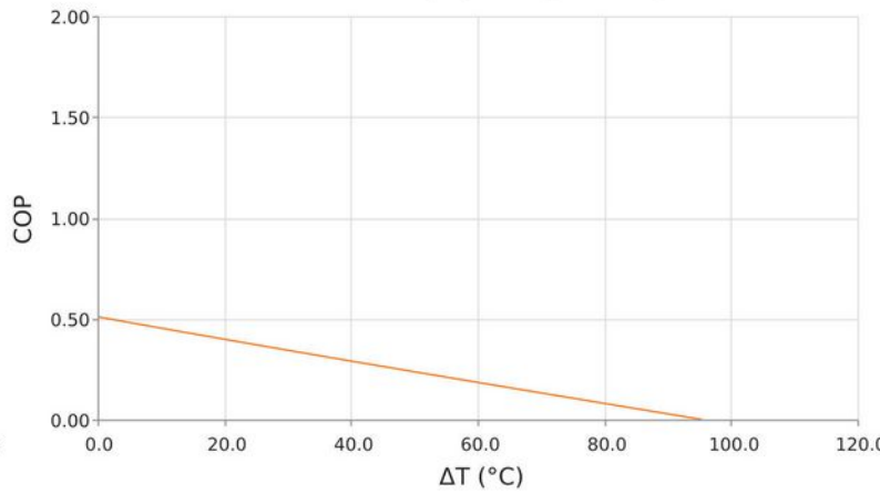
Coefficient of Performance ( COP = Q_c/P_{in} ) T_{hot} = 35^\circ C | I_{operating} = 1 Amps
