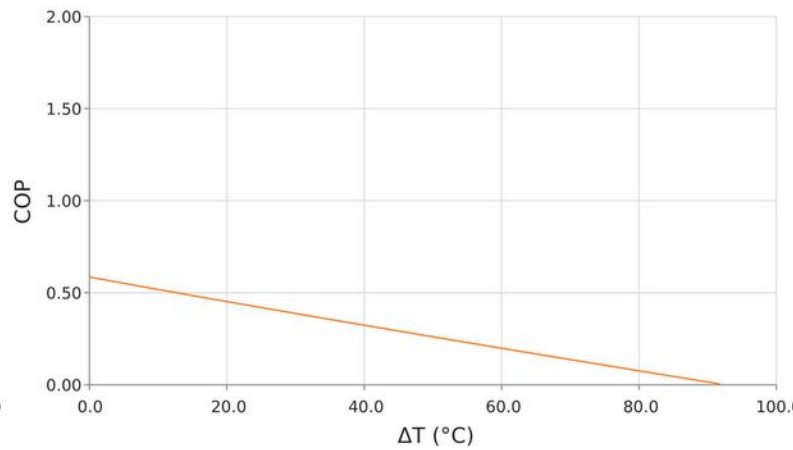
Coefficient of Performance ( COP = Q_c/P_{in} ) T_{hot} = 35^\circ\text{C} | I_{operating} = 0.9\text{ Amps}
