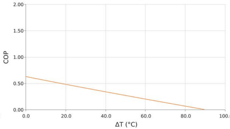
Coefficient of Performance ( COP = Q_c/P_{in} ) T_{hot} = 35^\circ C | loperating = 3.5 Amps
