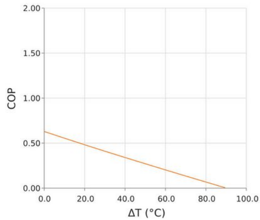
Coefficient of Performance (COP = Q_c/P_{in} ) T_{hot} = 35^\circ\text{C} | I_{operating} = 3.5 Amps
