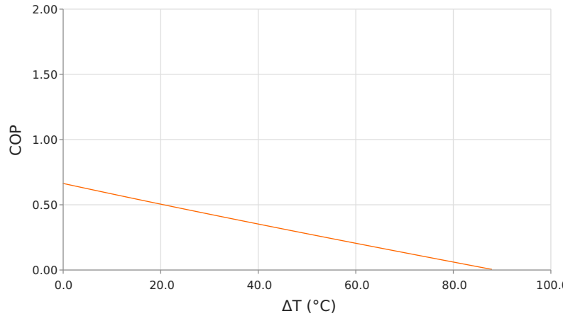
Coefficient of Performance (COP = Qc/Pin) Thot = 35 °C | Ioperating = 0.4 Amps
