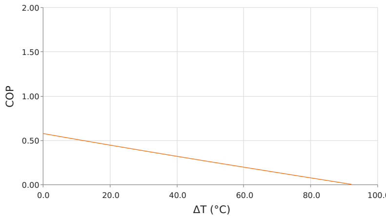
Coefficient of Performance (COP = Qc/Pin) Thot = 35 °C | Ioperating = 2.2 Amps
