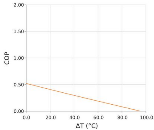
Coefficient of Performance (COP = Q_c/P_{in} ) T_{hot} = 35^\circ\text{C} | I_{operating} = 3.4 Amps
