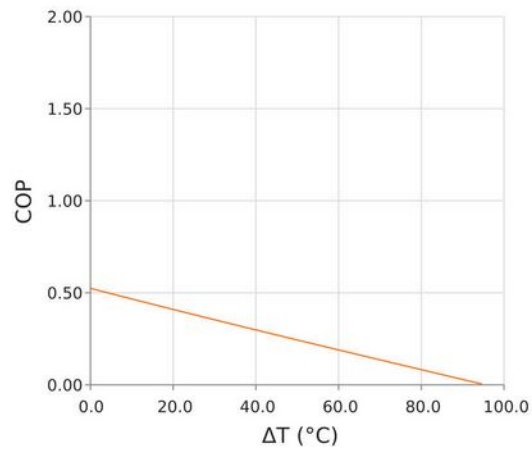
Coefficient of Performance (COP = Q_c/P_{in} ) T_{hot} = 35\text{ }^{\circ}\text{C} | I_{operating} = 8.2\text{ Amps}
