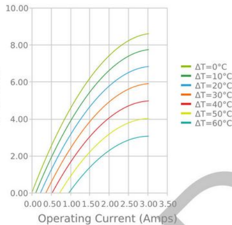
Heat Pumped at Cold Side T_{hot} = 27^\circ C
