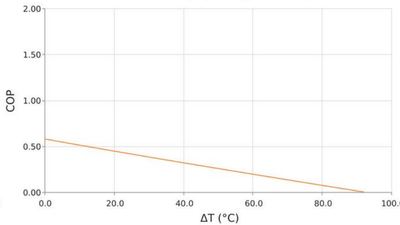
Coefficient of Performance ( COP = Q_c/P_{in} ) T_{hot} = 35^\circ C | I_{operating} = 2.3 Amps
