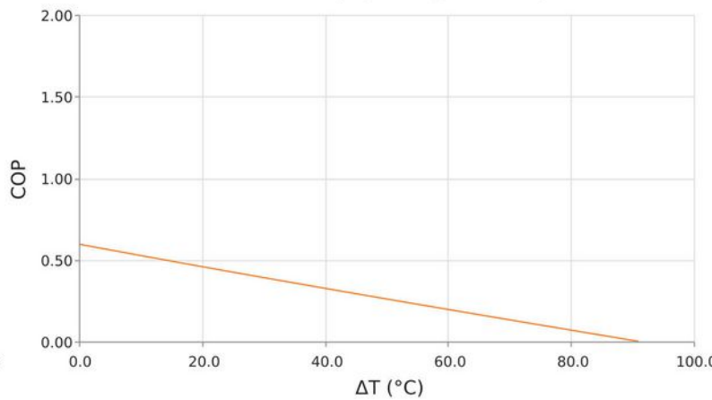
Coefficient of Performance ( COP = Q_c/P_{in} ) T_{hot} = 35^\circ C | I_{operating} = 5.4 Amps
