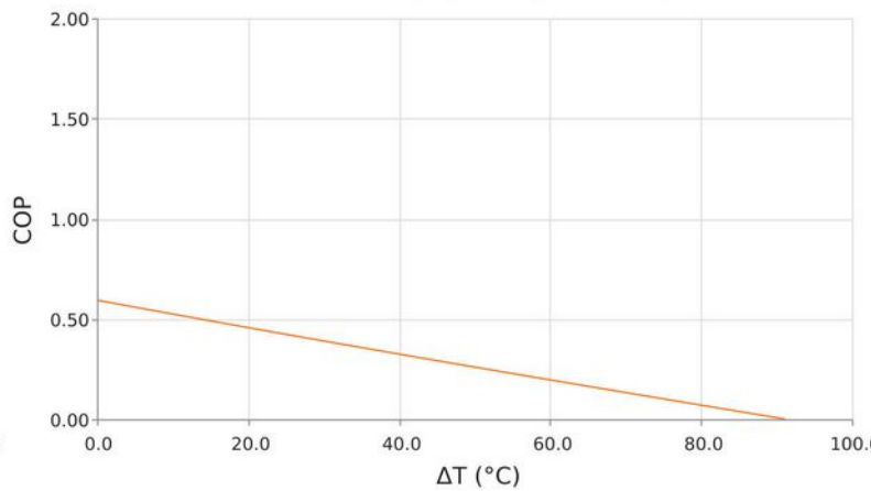
Coefficient of Performance ( COP = Q_c/P_{in} ) T_{hot} = 35^\circ C | I_{operating} = 3.9 Amps
