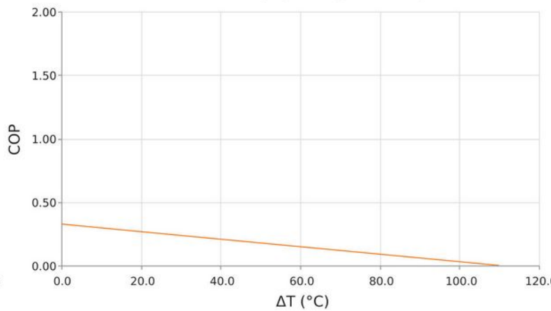
Coefficient of Performance ( COP = Q_c/P_{in} ) T_{hot} = 35^\circ C | Operating = 1.5 Amps
