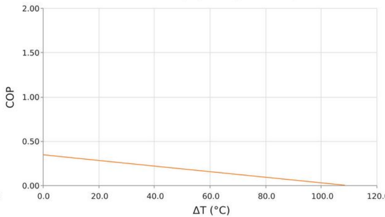
Coefficient of Performance ( COP = Q_c/P_{in} ) T_{hot} = 35^\circ C | I_{operating} = 3.1 Amps
