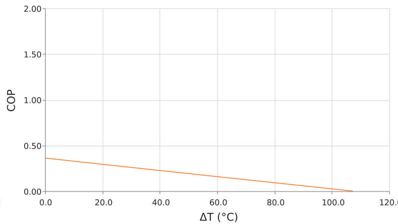
Coefficient of Performance (COP = Q_c/P_{in} ) T_{hot} = 35^\circ\text{C} | I_{operating} = 6.4 Amps
