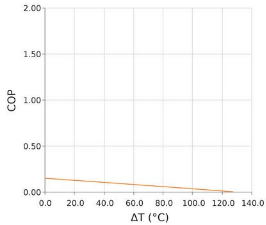
Coefficient of Performance (COP = Q_c/P_{in} ) T_{hot} = 35^\circ\text{C} | I_{operating} = 3.1 Amps
