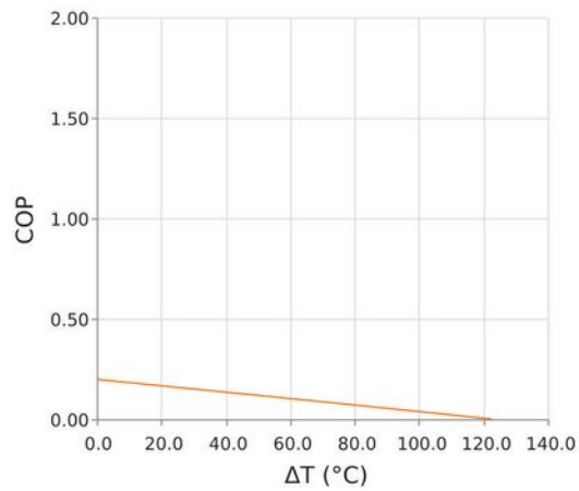
Coefficient of Performance (COP = Q_c/P_{in} ) T_{hot} = 35\text{ }^{\circ}\text{C} | I_{operating} = 1.5\text{ Amps}
