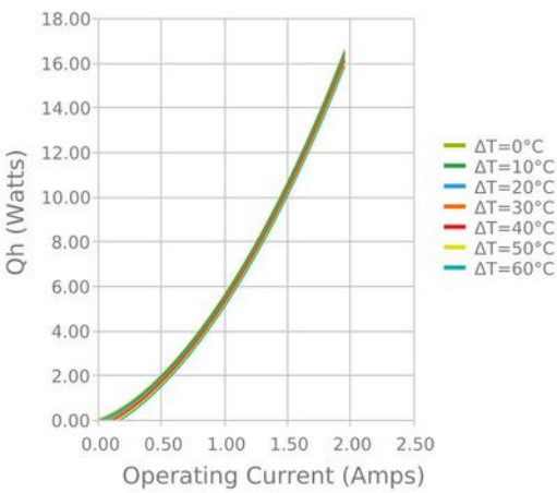
Total Heat Dissipated at Hot Side ( Q_h=Q_c+P_{in} ) T_{hot} = 27\text{ }^{\circ}\text{C}
