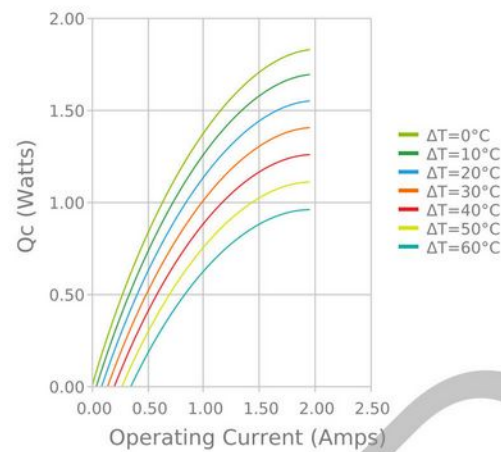
Heat Pumped at Cold Side T_{hot} = 27^\circ C
