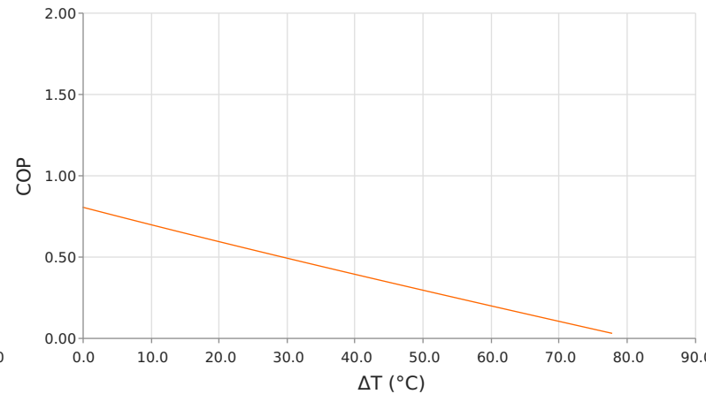
Coefficient of Performance ( COP = Q_c/P_{in} ) T_{hot} = 50\text{ }^{\circ}\text{C} | I_{operating} = 0.7\text{ Amps}
