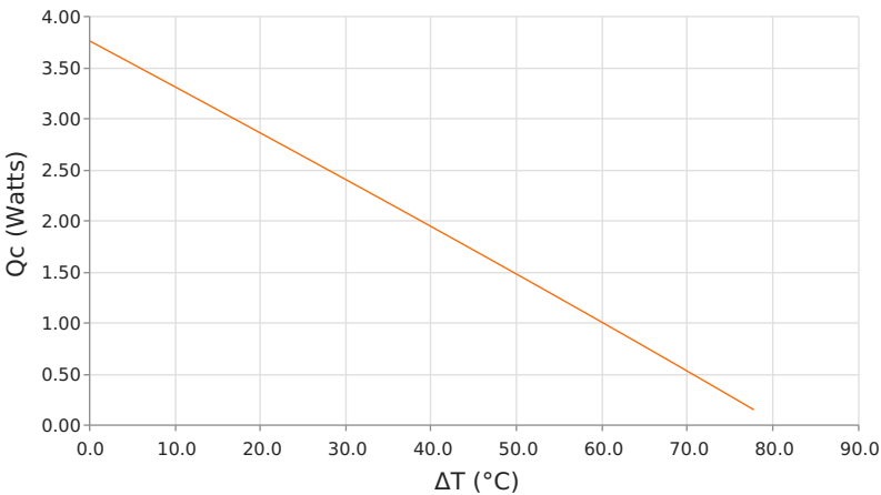
Heat Pumped at Cold Side ( Q_c ) T_{hot} = 50\text{ }^{\circ}\text{C} | I_{operating} = 0.7\text{ Amps}
