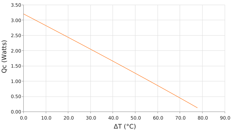
Heat Pumped at Cold Side ( Q_c ) T_{hot} = 50\text{ }^{\circ}\text{C} | operating = 1.3 Amps
