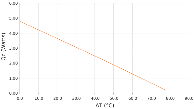
Heat Pumped at Cold Side (Qc) Thot = 50 °C | Ioperating = 1.6 Amps
