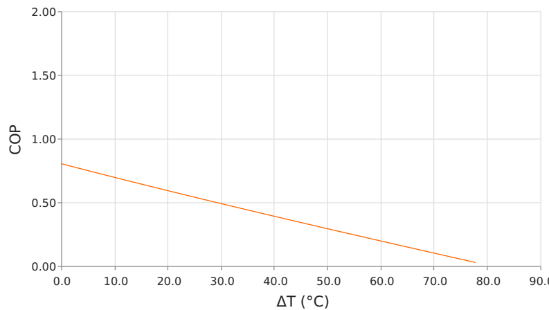
Coefficient of Performance ( COP = Q_c/P_{in} ) T_{hot} = 50\text{ }^{\circ}\text{C} | operating = 1.6 Amps
