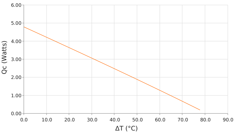
Heat Pumped at Cold Side ( Q_c ) T_{hot} = 50\text{ }^{\circ}\text{C} | operating = 1.6 Amps
