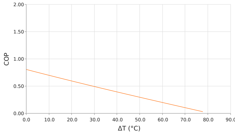
Coefficient of Performance ( COP = Q_c/P_{in} ) T_{hot} = 50^\circ C | operating = 1.7 Amps
