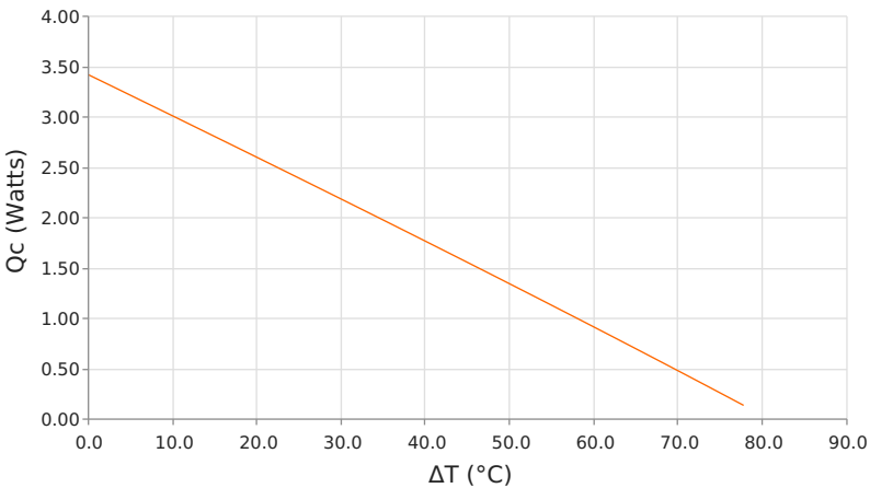
Heat Pumped at Cold Side ( Q_c ) T_{hot} = 50^\circ C | operating = 1.7 Amps
