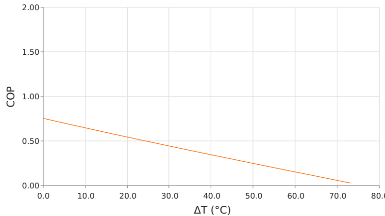
Coefficient of Performance (COP = Q_c/P_{in} ) T_{hot} = 50^\circ\text{C} | operating = 12.5 Amps
