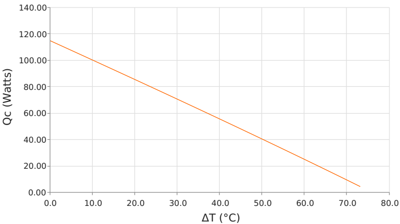
Heat Pumped at Cold Side ( Q_c ) T_{hot} = 50^\circ\text{C} | operating = 12.5 Amps
