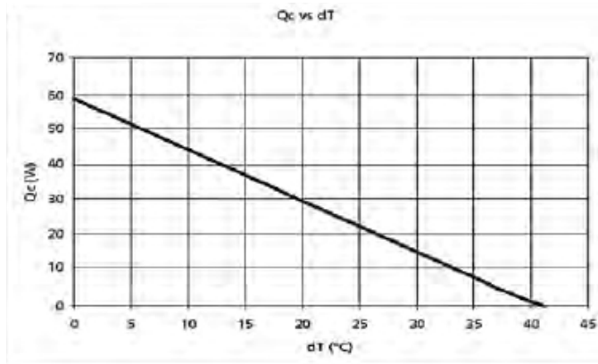
PERFORMANCE CURVE
